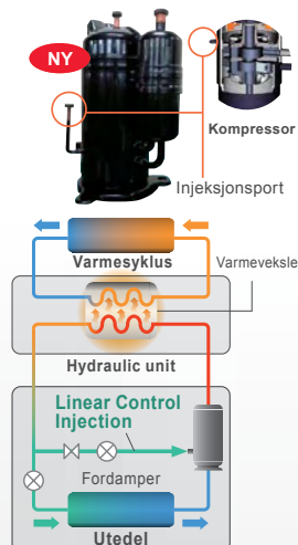
Co-axial varmeveksler
